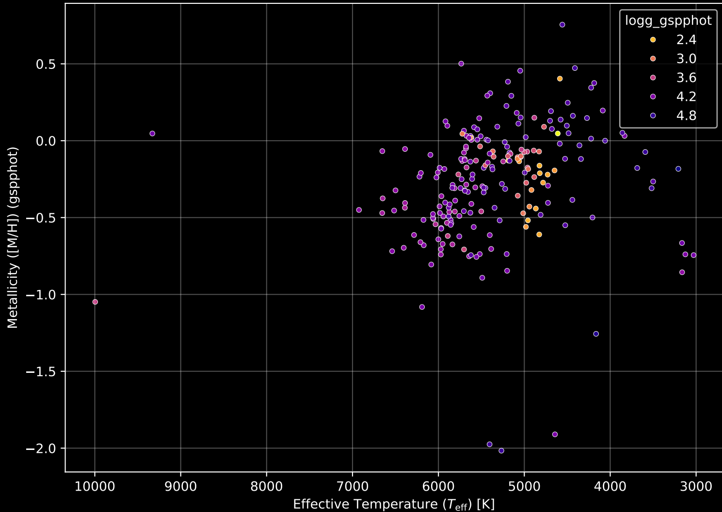
APOGEE DR17 Field: [222+71_MGA] Stellar Population Parameters (n= 221)
