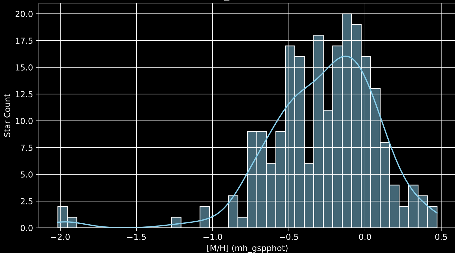
APOGEE DR17 Field: [222+71_MGA [M/H] (mh_gspphot) (n= 219)
