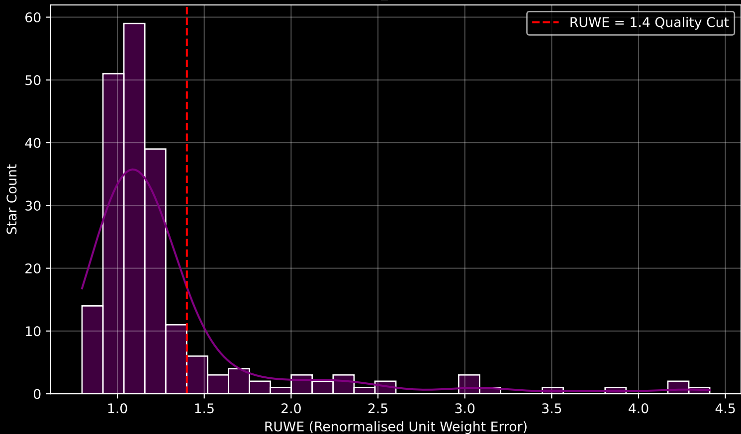
GAPOGEE DR17 Field [222+71_MGA] RUWE Distribution (n= 210)
