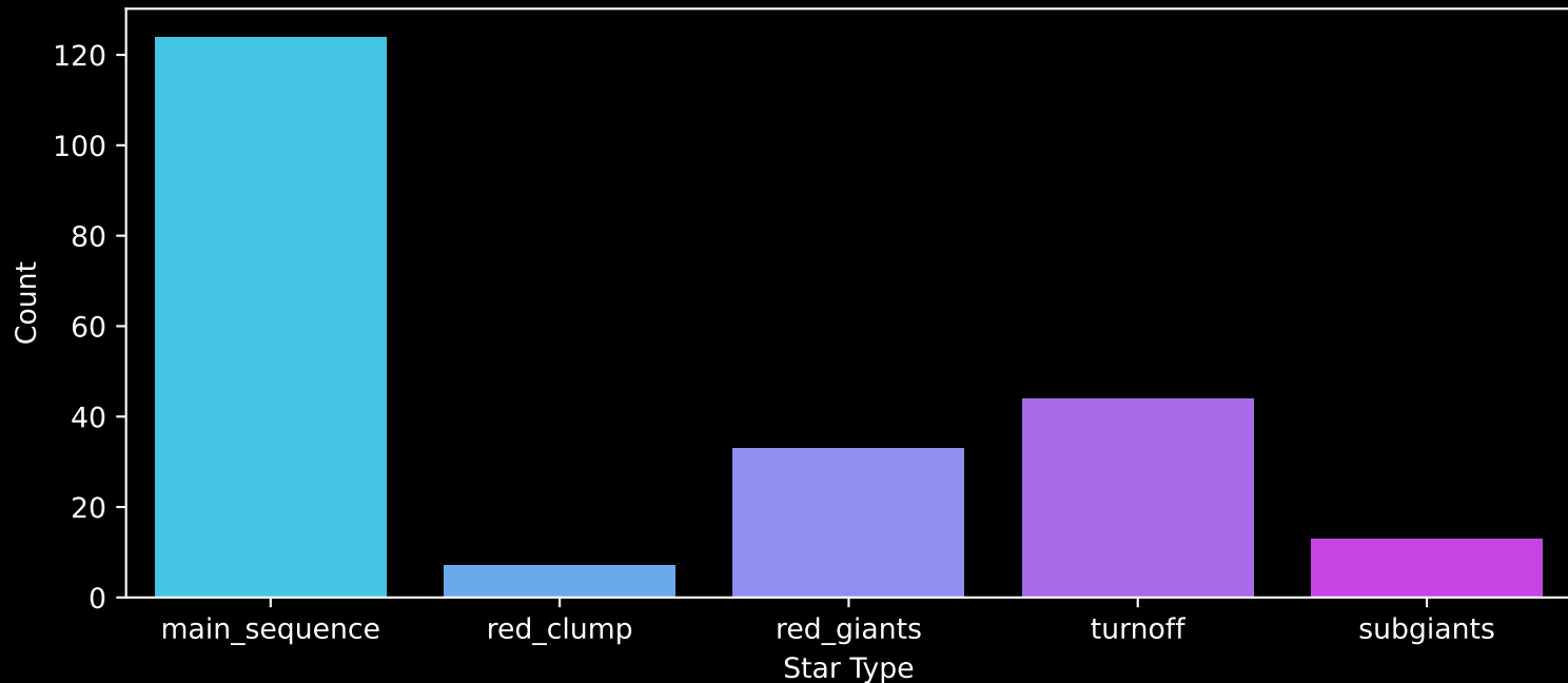
APOGEE DR17 Field: [222+71_MGA] Count plot of Star Type
